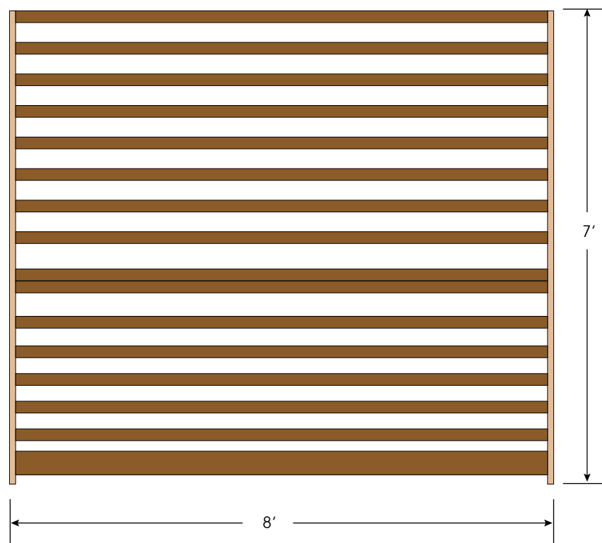
Bank Framing Top View
