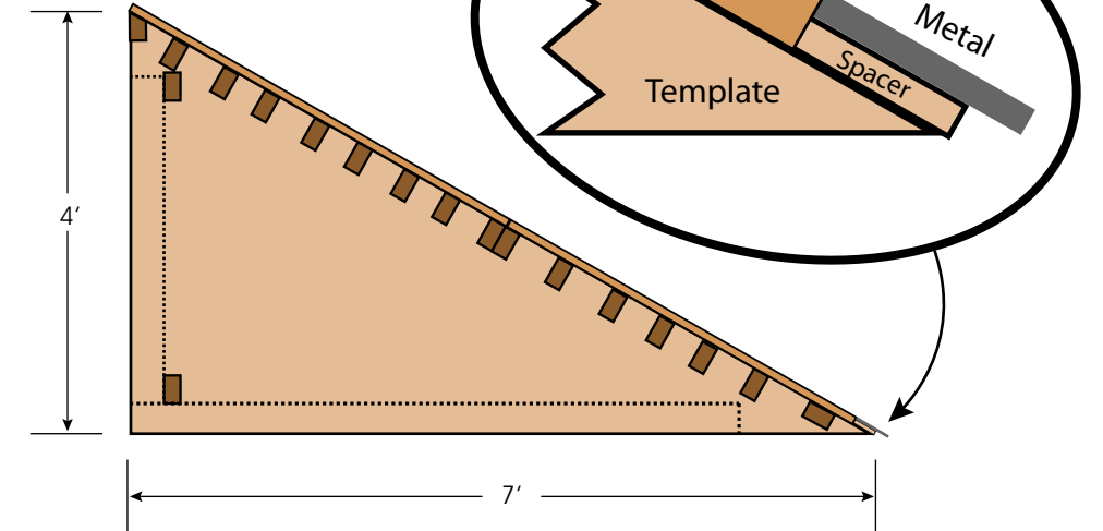
Bank Side View
